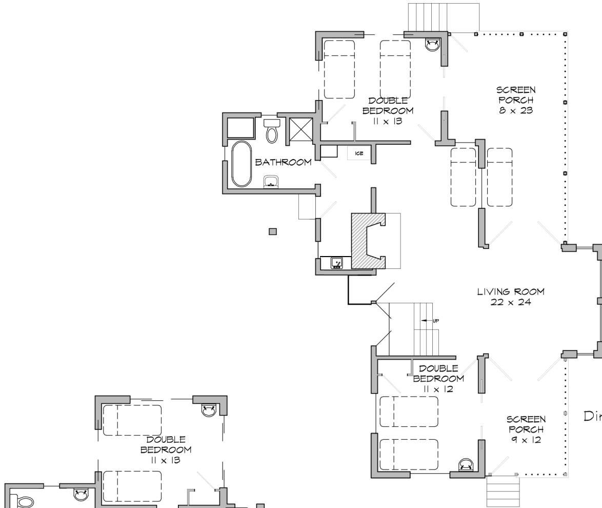
FIRST FLOOR PLAN Scale: 3/32" = 1'
