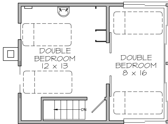
SECOND FLOOR PLAN Scale: 1/8" = 1'
