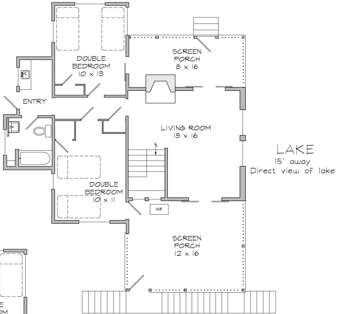
FIRST FLOOR PLAN Scale: 1/8" = 1'
